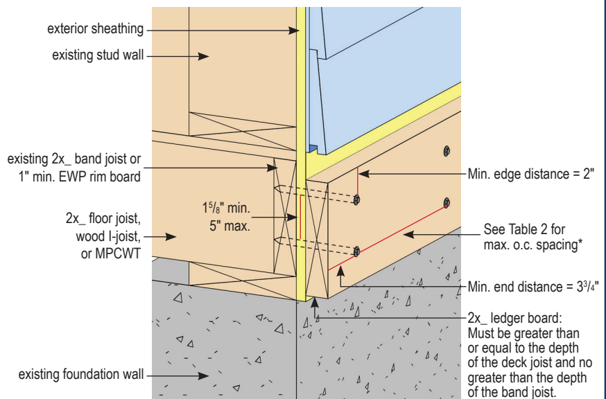
FIGURE 1. Deck Connection with 3/8" Diameter Ledger Board Screws
